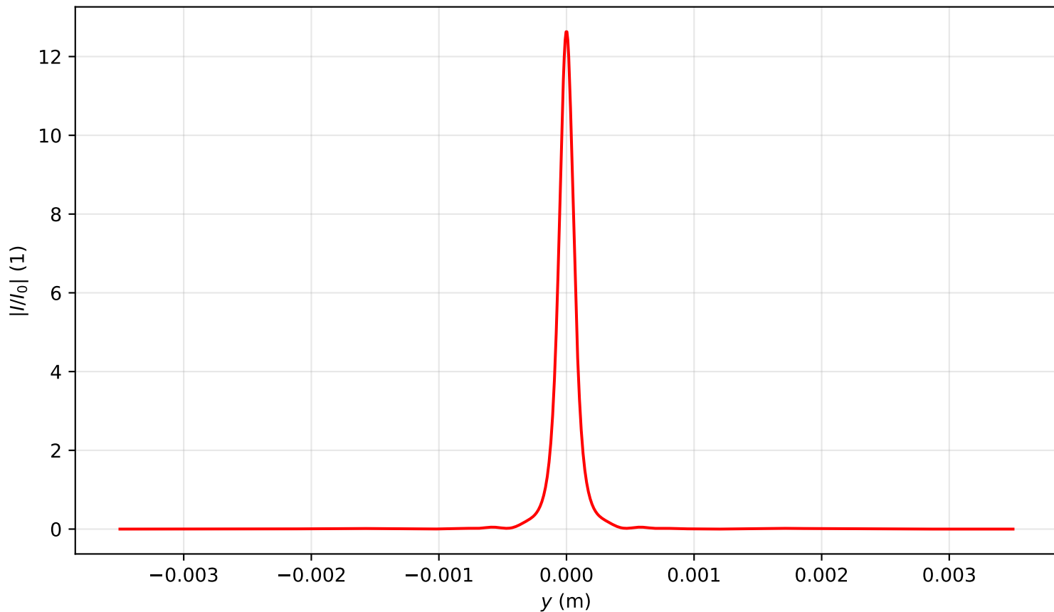
Intensity profile I(x=0, y, z=2.866)/I_0 , P_{in}=2.0P_{cr} , artificial time
